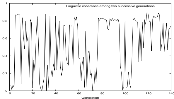
Figure 6: Linguistic coherence among two successive generations.
