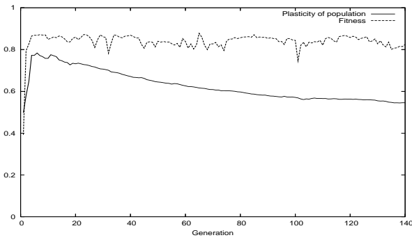
Figure 4: Fitness and plasticity of population.
