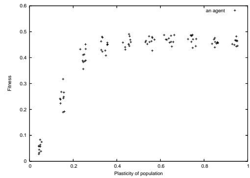
Figure 7: Correlation diagram of fitness and plasticity of population.
