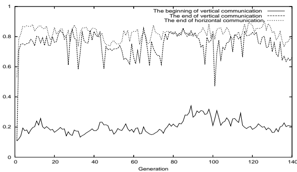
Figure 5: Linguistic coherence among the same generation.
